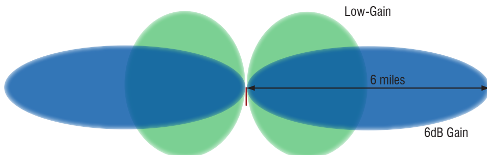
Increasing the gain of omni-directional antennas results in less energy sent vertically and more energy sent horizontally, extending the range.
