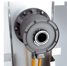
Save valuable installation space by using the hollow shaft diameter for hoses and cables.
