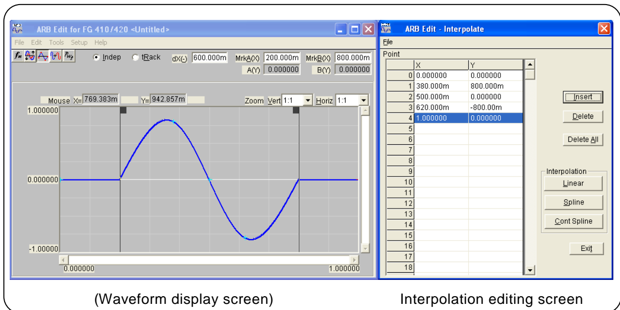
Figure 5-4 Interpolation Editing Screen
