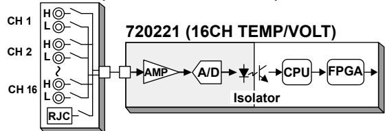
701953 (16CH SCANNER BOX)
