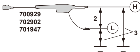
Direct input (cable that does not comply with the safety standards)
