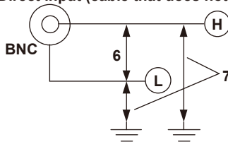
Direct input (cable that does not comply with the safety standards)
