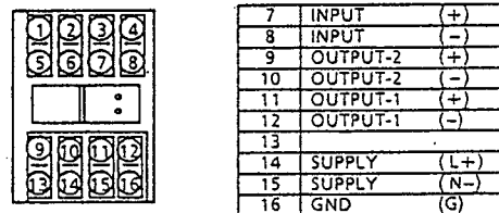
Fig.9 Terminal Arrangement
