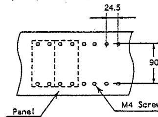
Fig.8 Panel (Wall) Mounting Dimension
