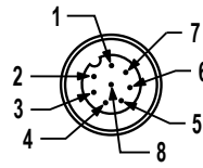
Euro-style Male Pinouts
