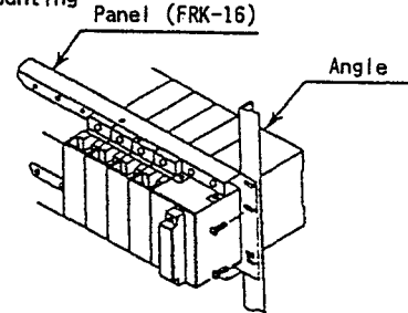
Fig.1 Rack Mounting
