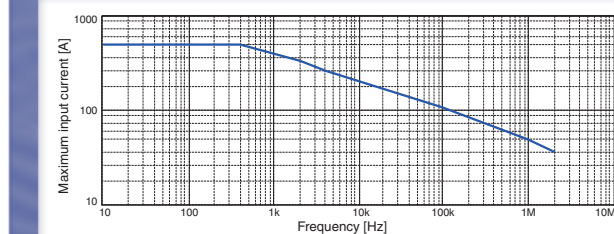
Fig.11 Current derating VS. frequency
