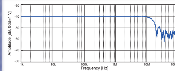
Fig.7 Frequency characteristics (typical)
