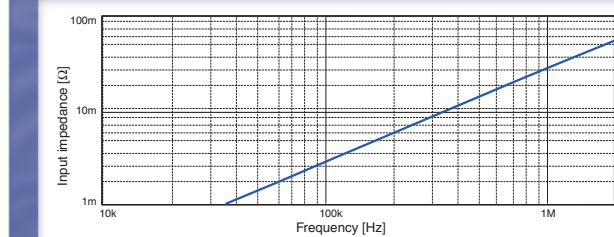
Fig.12. Input impedance (typical)
