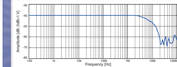
Fig.10 Frequency characteristics (typical)
