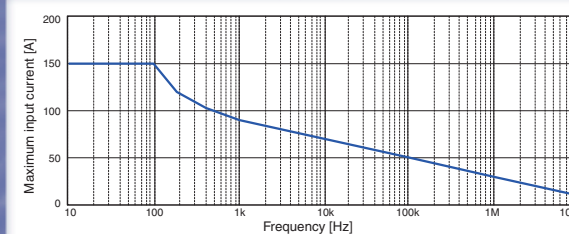
Fig.8 Current derating VS. frequency
