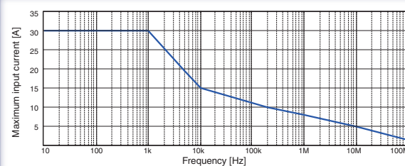
Fig.5 Current derating VS. frequency
