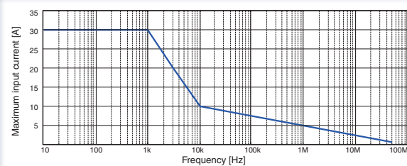
Fig.2 Current derating VS. frequency
