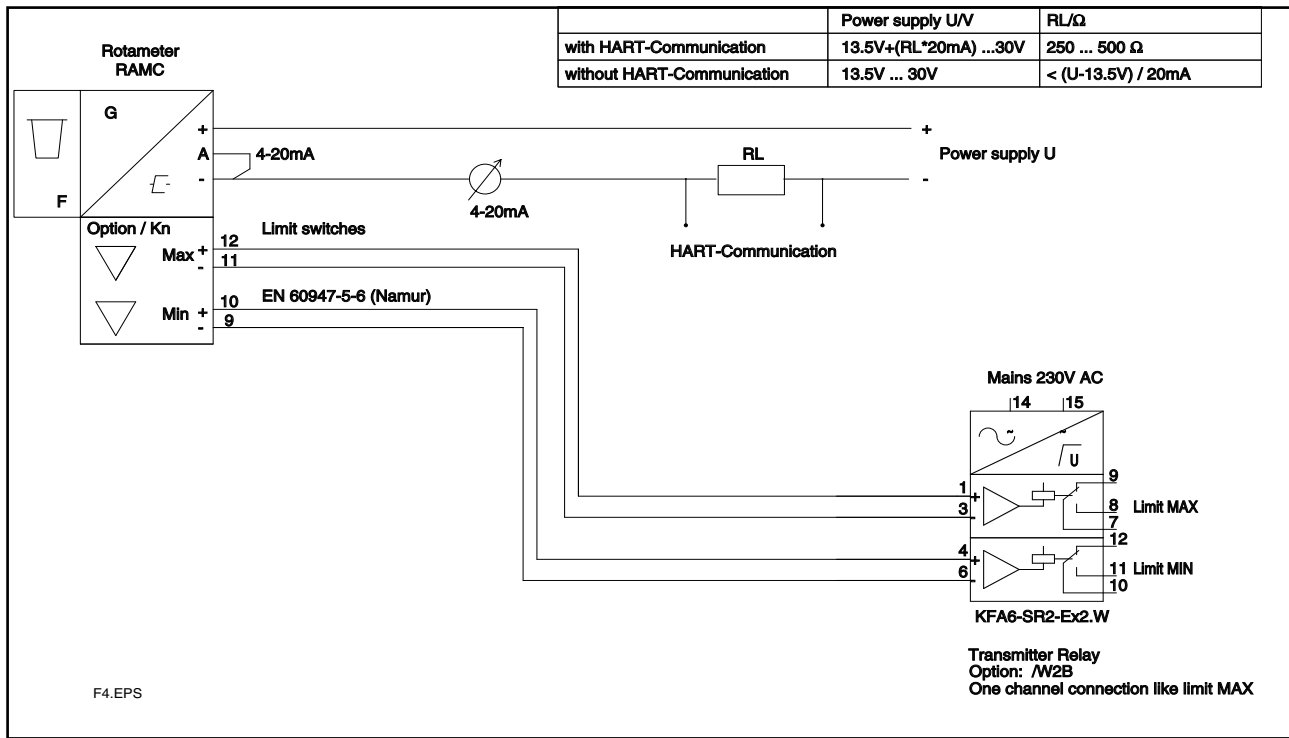
Fig. 3-7 RAMC 2-wire unit with HART-communication, with limit switches and transmitter relay
