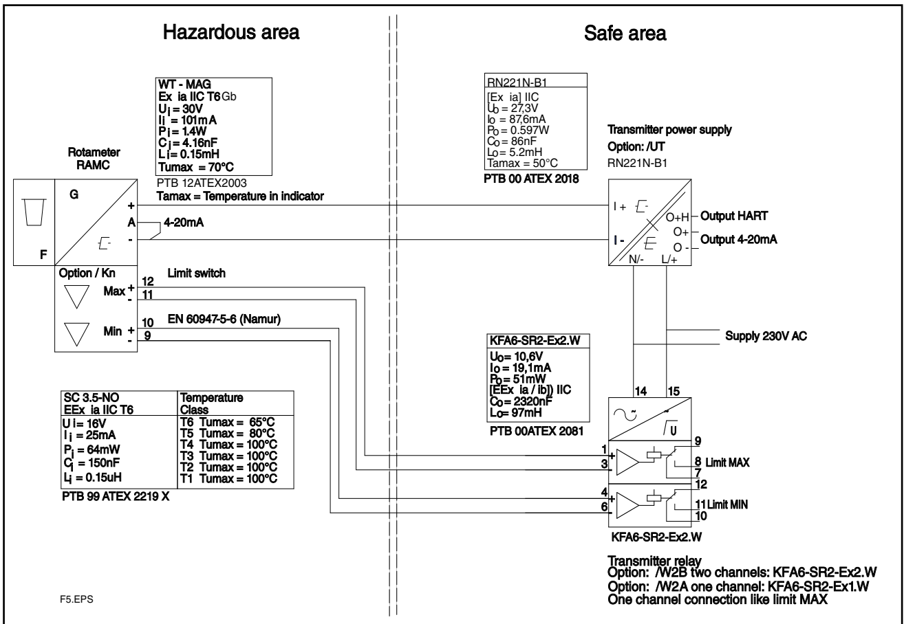
fig. 9-4 Intrinsic safe version according ATEX (option /KS1 or /KS2) : RAMC 2- wire unit with power supply, inductive limit switches and transmitter relay
