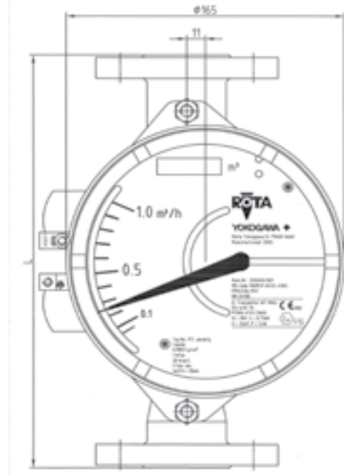
Fig. 9-8. Front view RAMC type 91
