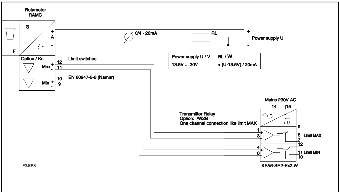
Fig. 3-4 RAMC 3-wire unit with limit switches and transmitter relay
