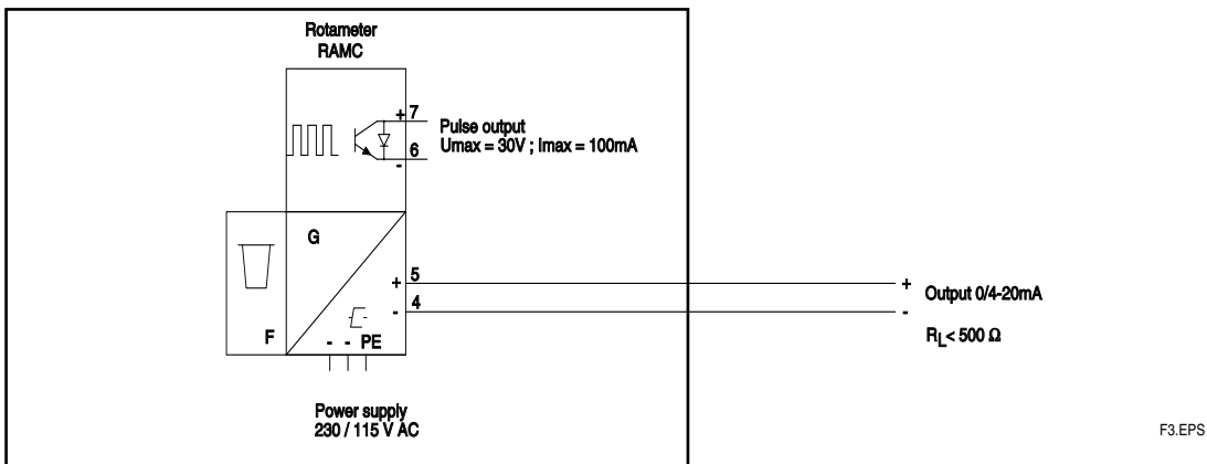
fig. 9-3 RAMC 4-wire unit with pulse output
