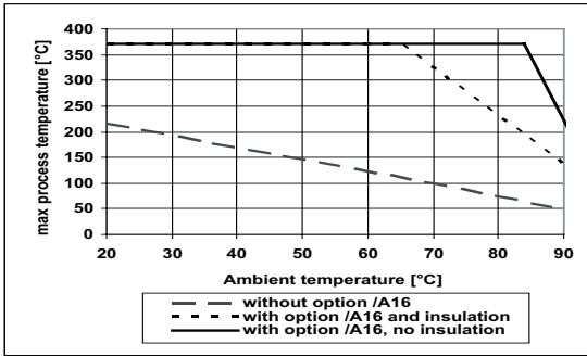
fig. 7a RAMC : - type 90 / 91 - only with indicator
