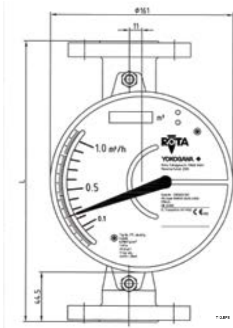
Fig. 9-7 Front view RAMC type 90
