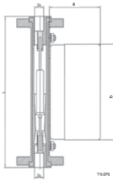
Fig. 9-10 RAMC metal measuring tube with lining
