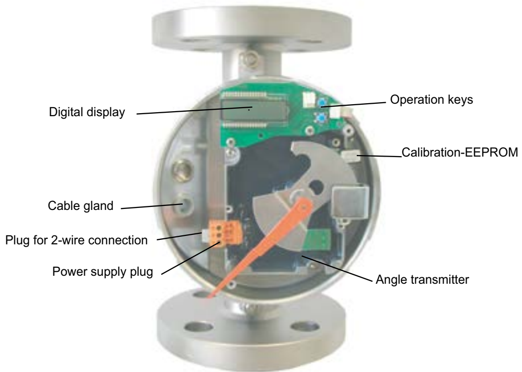
Fig. 3-1 2-wire unit
