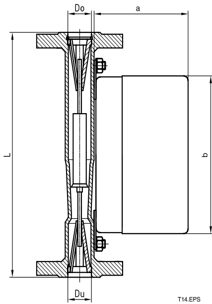
Fig. 9-13 RAMC metal measuring tube
