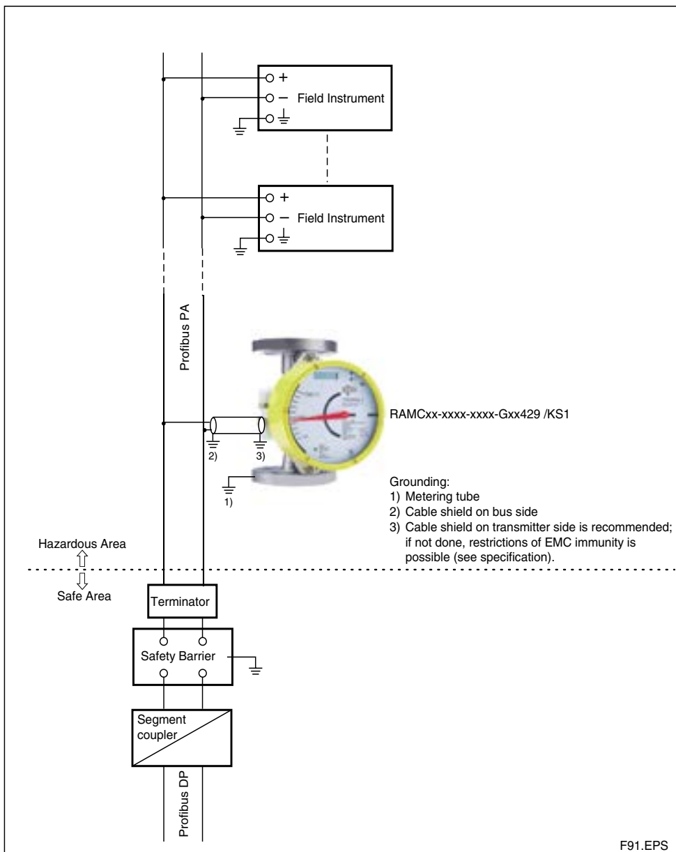
fig. 9-6 RAMC Profibus PA - communication
