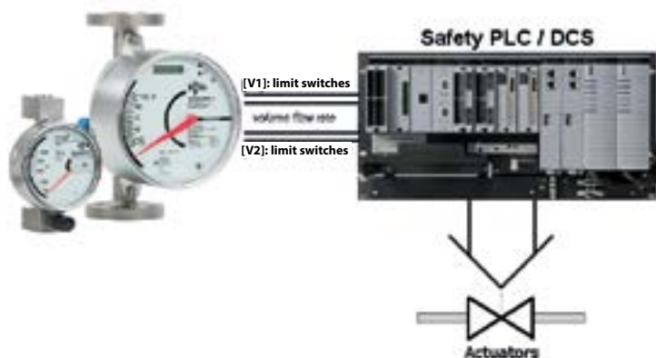
Figure A2.1 Example Safety Instrumented Function
