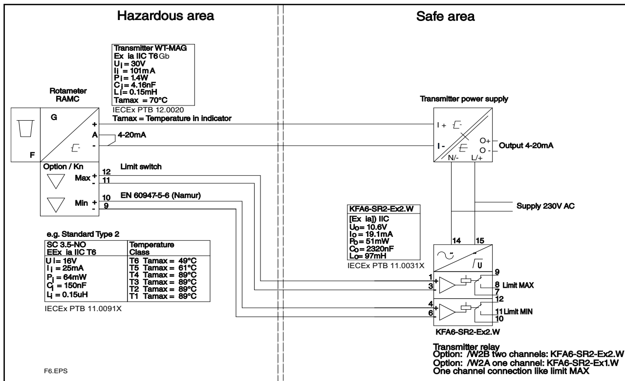
Fig. 10.2 Ex-Version according IECEx (Option /ES1) with electronic transmitter, power supply and limit switches with transmitter relay
