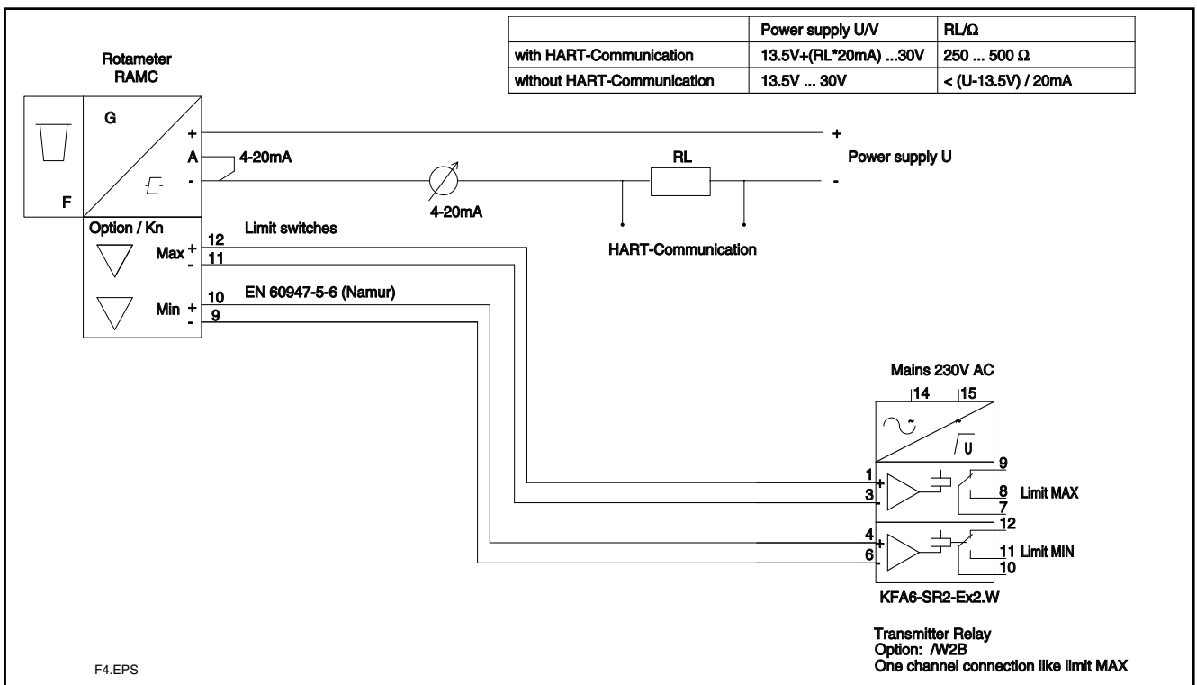
fig. 9-5 RAMC 2- wire unit with HART-communication, inductive limit switches and transmitter relay
