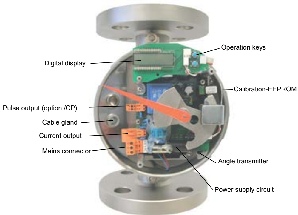
Fig. 3-2 4-wire unit
