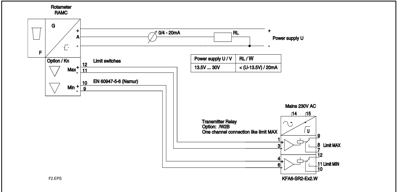
fig. 9-2 RAMC 3- wire unit with inductive limit switches and transmitter relay
