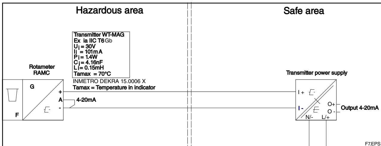
Fig. 10.3 Ex-Version according INMETRO (Option /US1) with electronic transmitter, power supply
