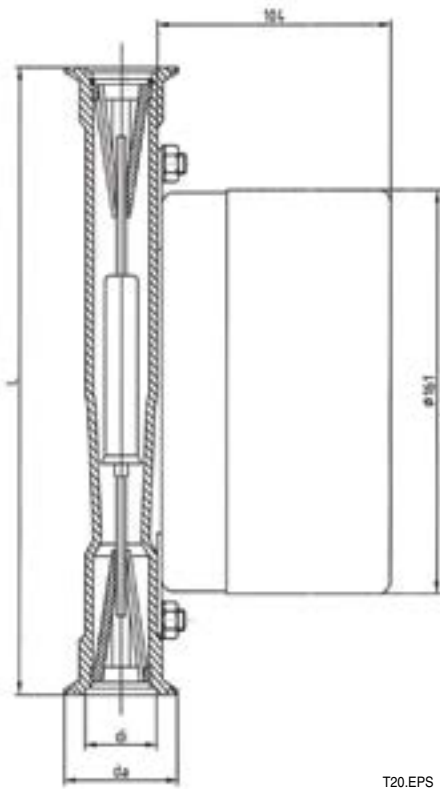
fig. 9-15 RAMC with connection S4
