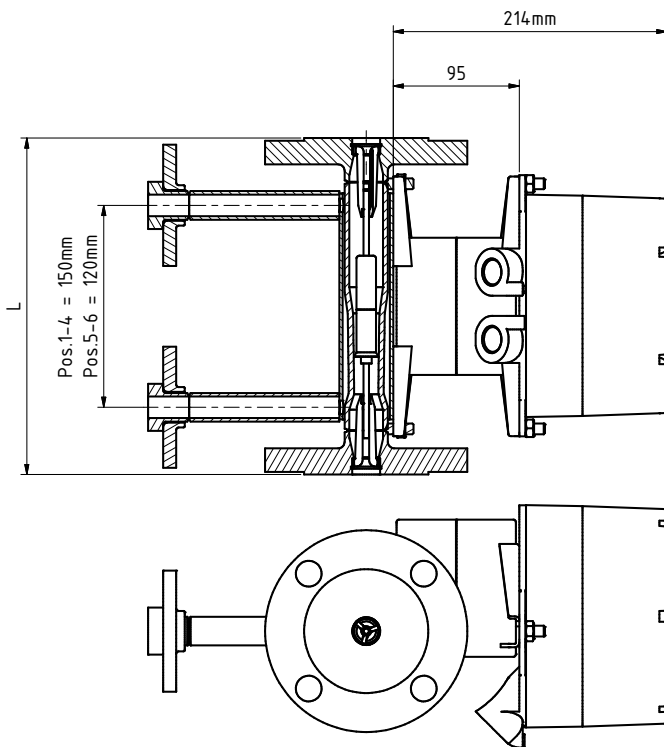
Fig. 9-11 RAMC type 91 and option /A16 and /T2
