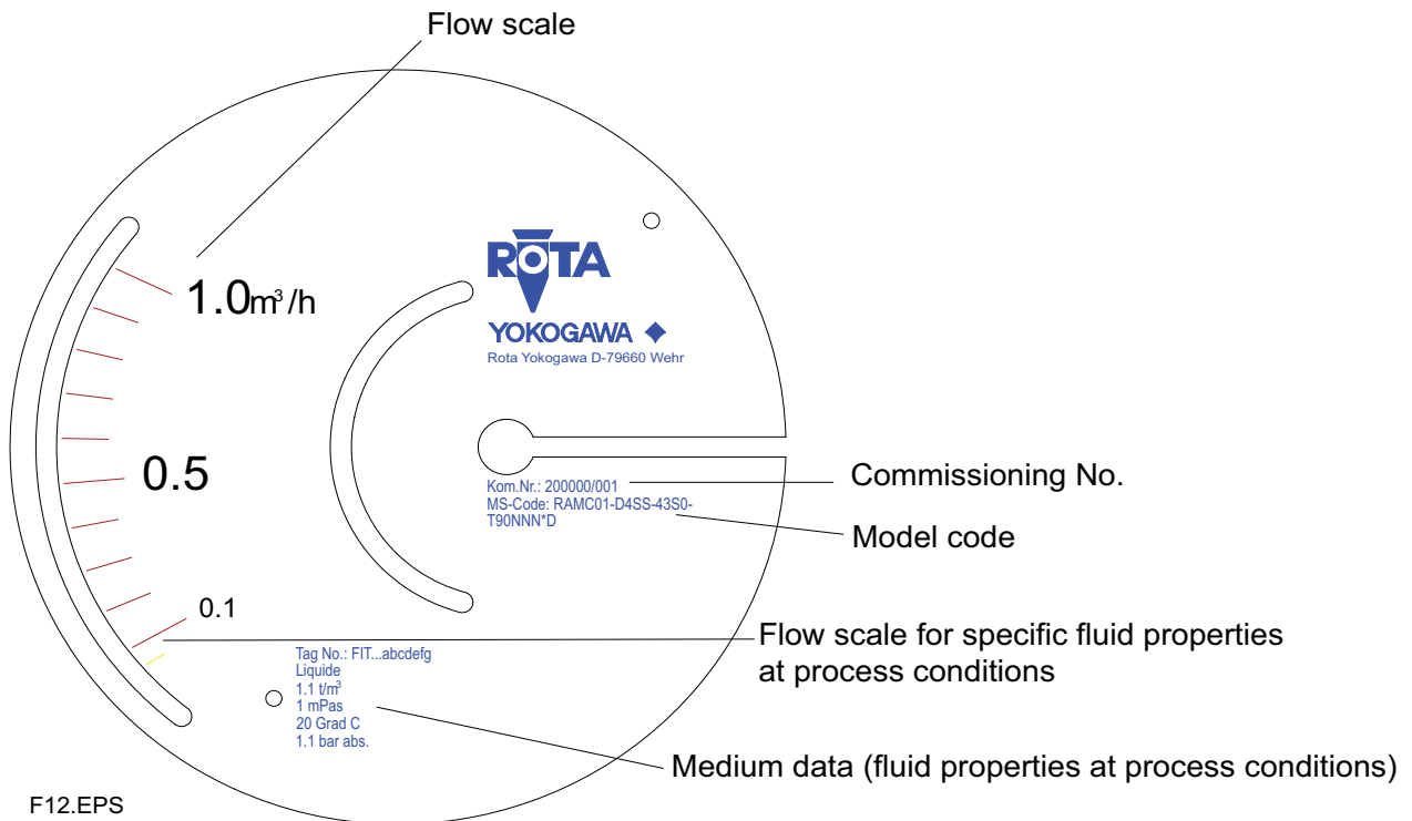
Fig. 1-4 Scale example for -T -type
