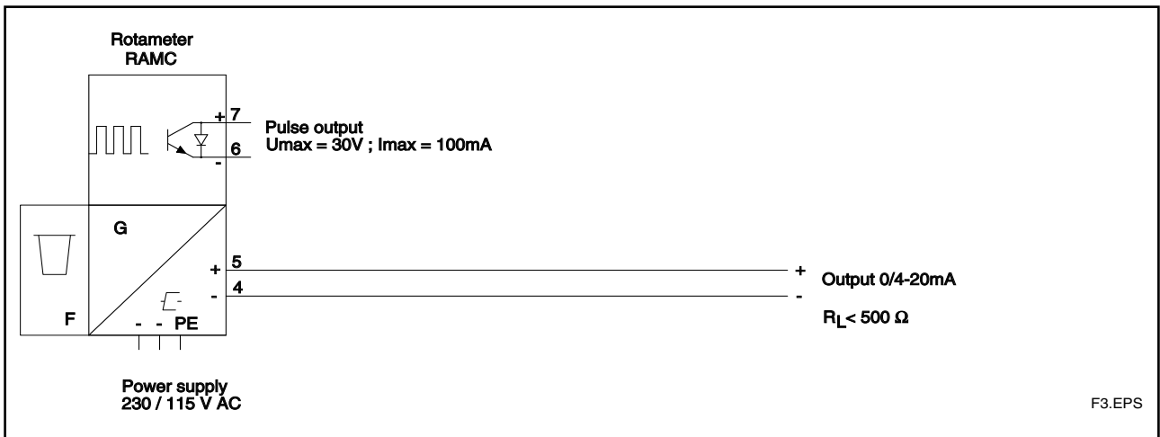
Fig. 3-5 RAMC 4-wire unit with pulse output
