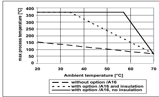
fig. 7b RAMC : - type 90 / 91 - with limit switches - with electronic transmitter
