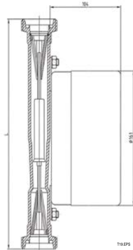
Fig. 9-14 RAMC with connection S2
