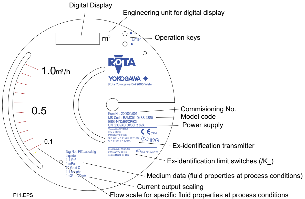
Fig. 1-3 Scale example for -E / -H / -J -type (electronic transmitter)
