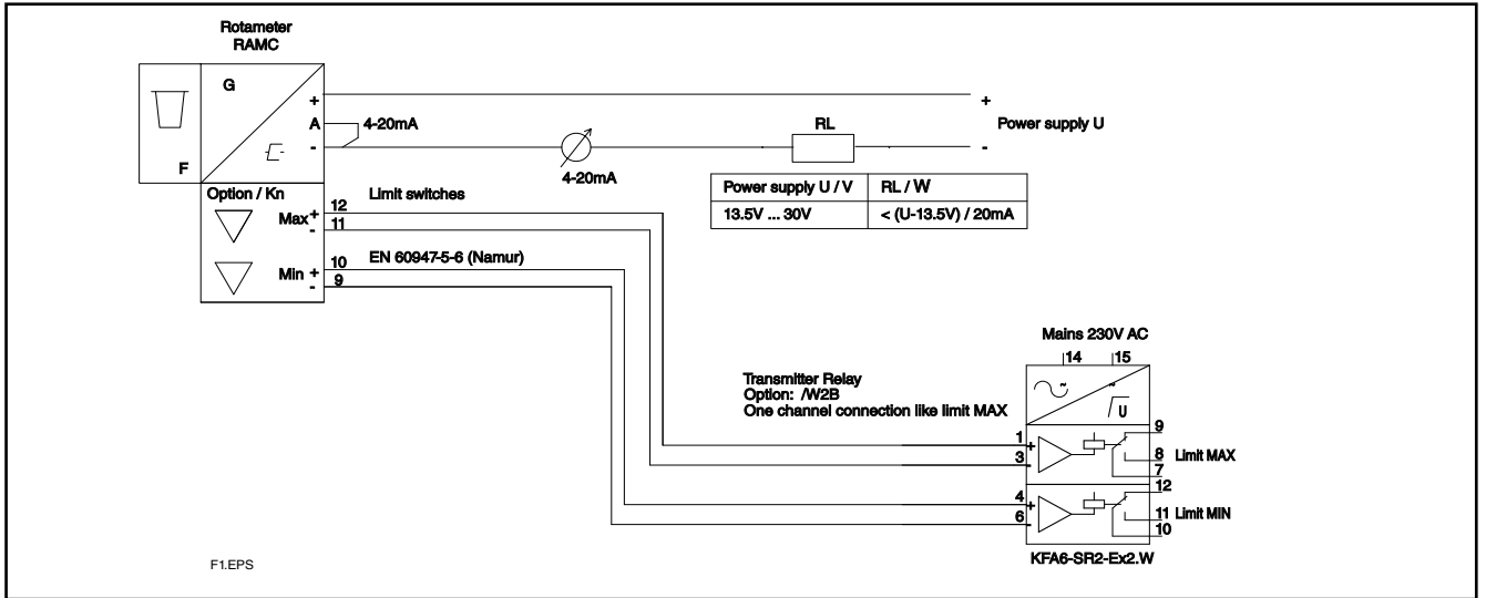
fig. 9-1 RAMC 2- wire unit with inductive limit switches and transmitter relay
