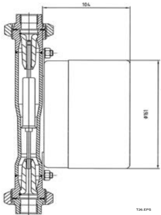
Fig. 9-12 RAMC with connection R4 / T4
