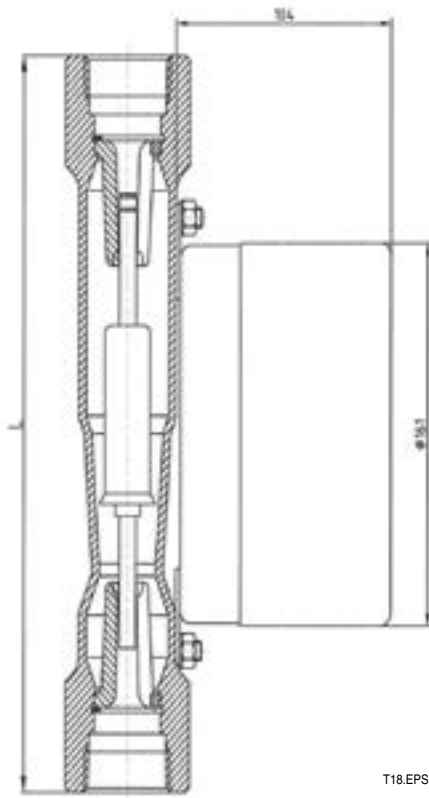
Fig. 9-13 RAMC with connection T6/ G6
