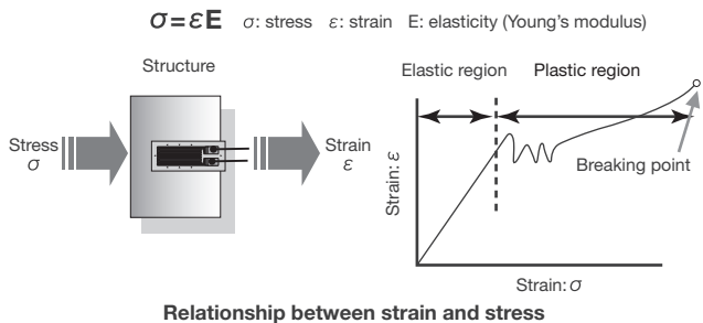
Relationship between strain and stress
