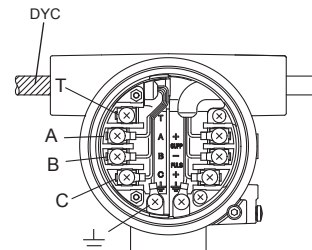
Remote type converter (DYA)
