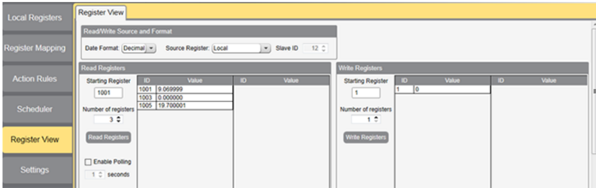
Figure 2. DXM Configurator showing the local floating point registers of the Decagon 5TE
