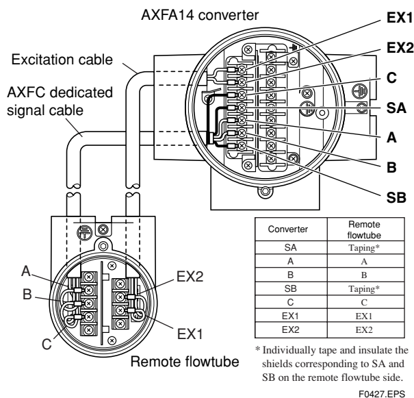
Figure 4.2.12 Wiring Diagram
