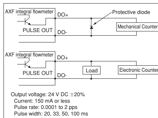
Figure 4.1.12 Active Pulse Output Connection (Optional code EM)
