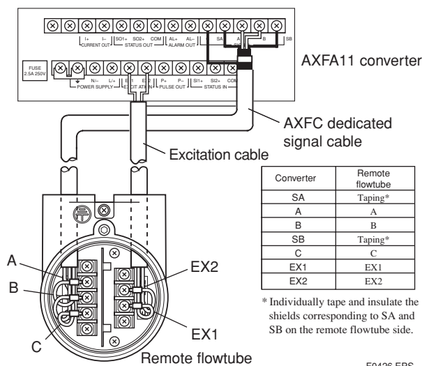
Figure 4.2.11 Wiring Diagram
