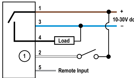
Figure 4: PNP
