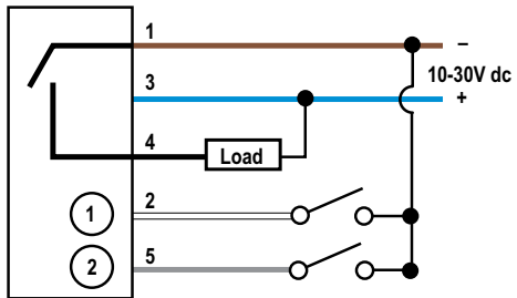
Figure 1: NPN
