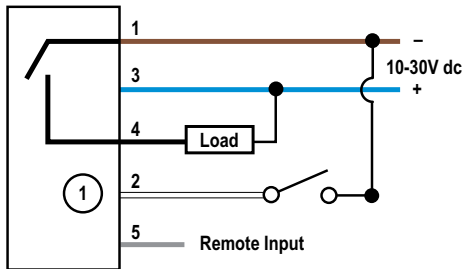
Figure 3: NPN
