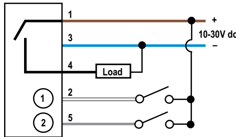
Figure 2: PNP
