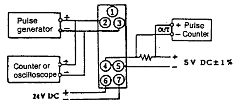
Calibration equipment wiring
