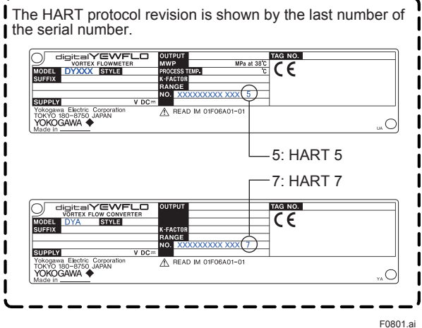
Figure 8.1 Name Plate
