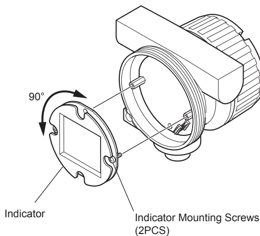
Figure 11.1 Removing and Reinstalling the Indicator
