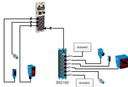
Figure 3: SIG100 as IO-Link Slave
