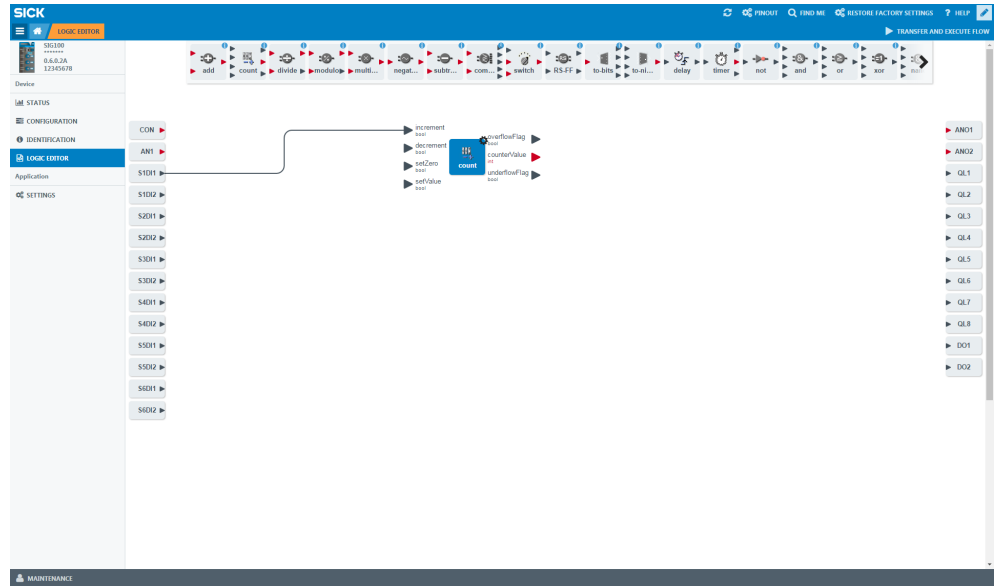
Figure 14: Possible connections
