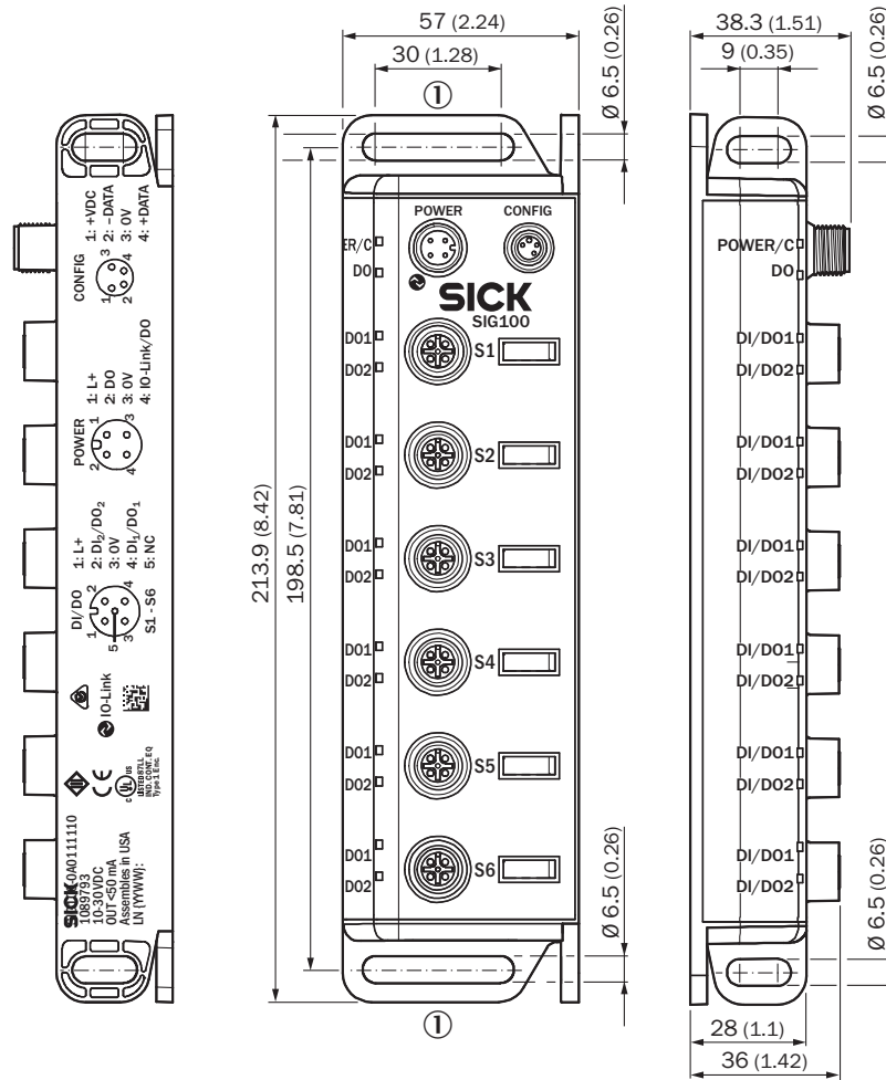
Figure 21: Dimensional drawing (dimensions in mm (inch))
