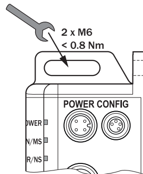
Figure 5: Mounting
