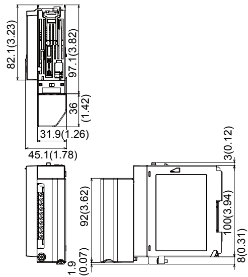
Clamp terminals
