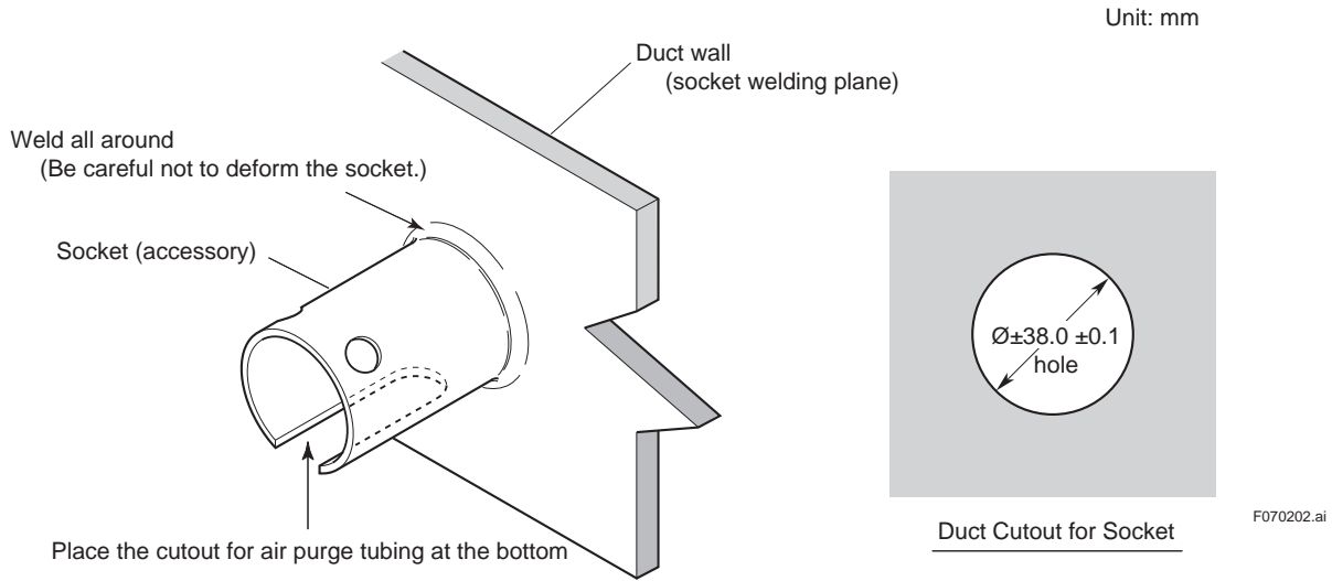
Connection Port for Socket Mounting Model
