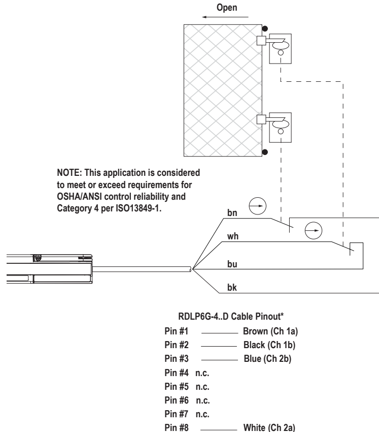
Figure 52. Monitoring two positive-opening safety switches
