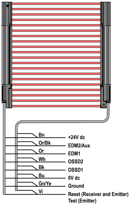
Figure 33. Individual Cordsets
