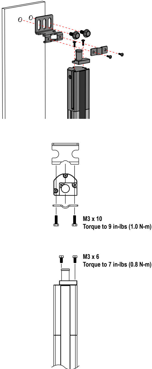
Figure 19. End-mount hardware attachment
