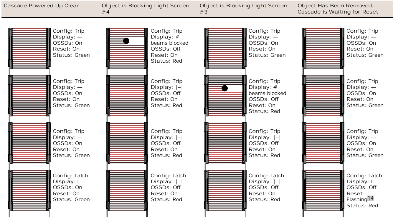
Figure 41. Cascade Indicator Status Conditions
