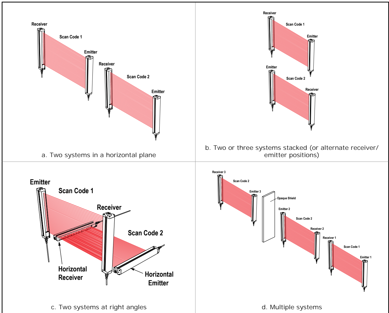
Figure 14. Installation of Multiple Systems
