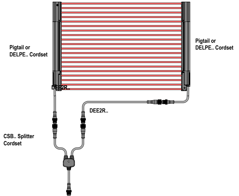
Figure 34. Splitter Cordsets
