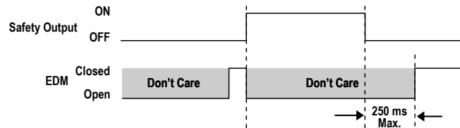
Figure 30. One-channel EDM status, with respect to safety output
