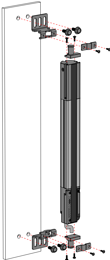
Figure 15. End-Mount Brackets
