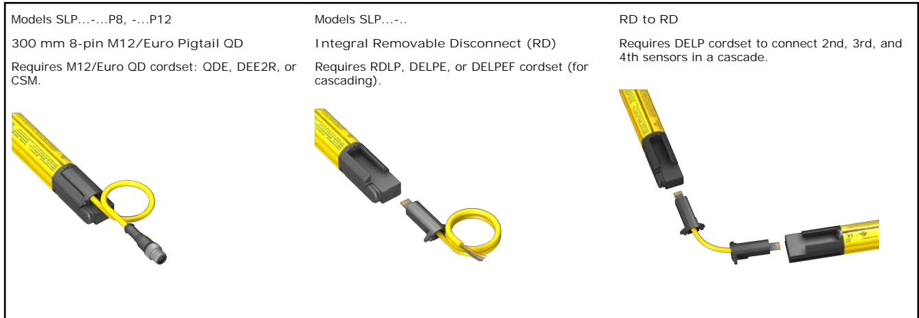
Figure 45. EZ-SCREEN LP Low Profile Safety Light Screen Connection Options
