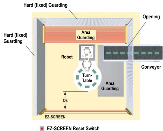
Figure 9. An example of supplemental safeguarding
