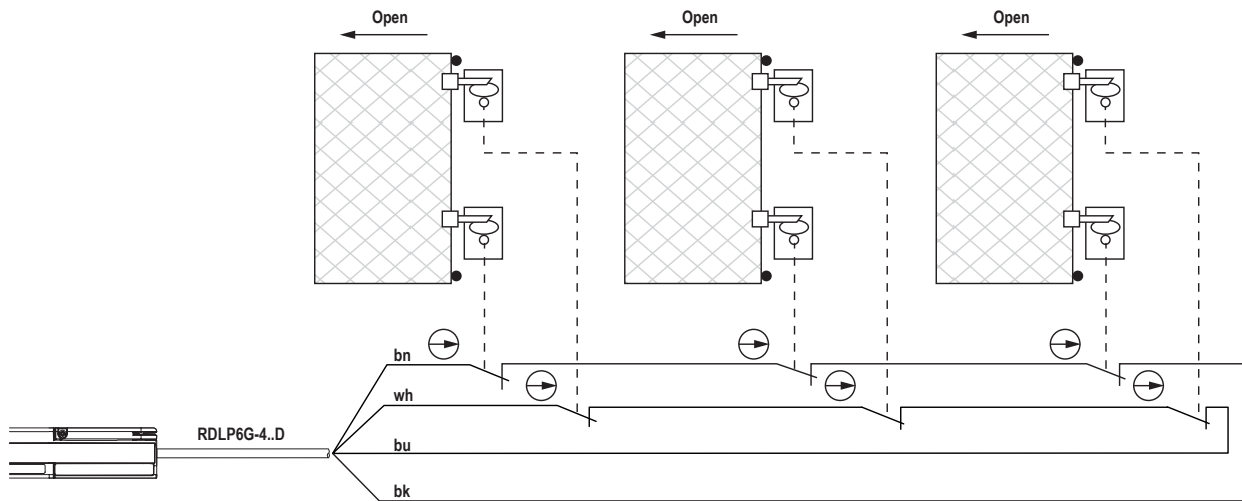
RDLP6G-4..D Cordset Pinout* Brown – Ch 1a White – Ch 2a Blue – Ch 2b Black – Ch 1b
