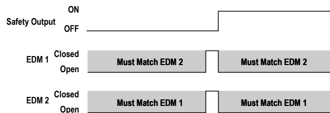
Figure 32. Two-channel EDM status, with respect to safety output
