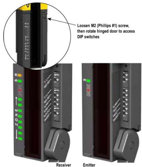
Figure 40. Accessing the configuration switches
