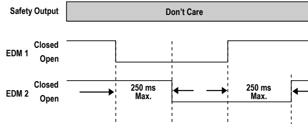
Figure 31. Two-channel EDM, timing between channels
