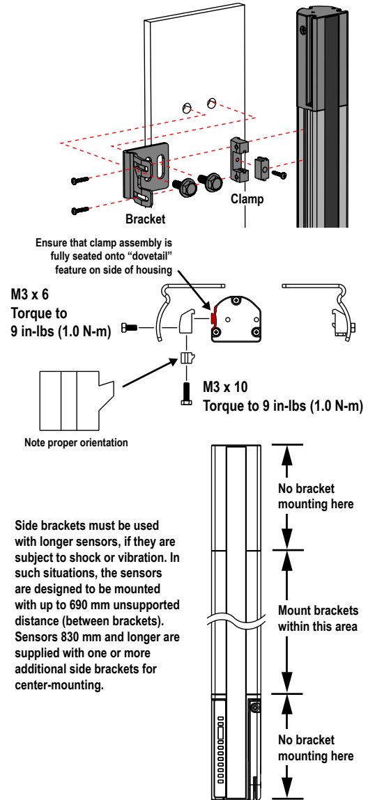
Figure 20. Side-mount hardware attachment
