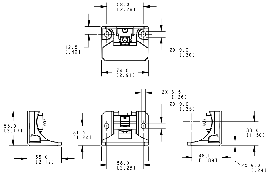
Side-Mount Bracket LPA-MBK-16
