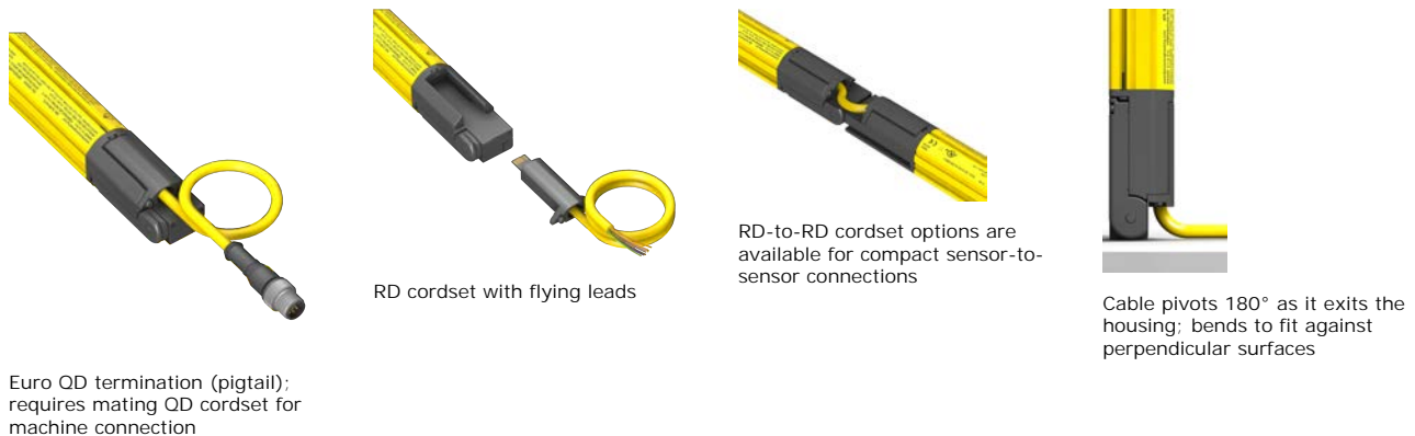
Figure 2. EZ-SCREEN LP removable-disconnect (RD) cordsets
