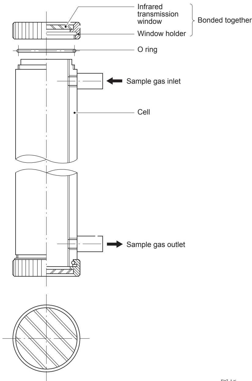
Fig. 6-1 Structure of sample cell (pipe cell)
